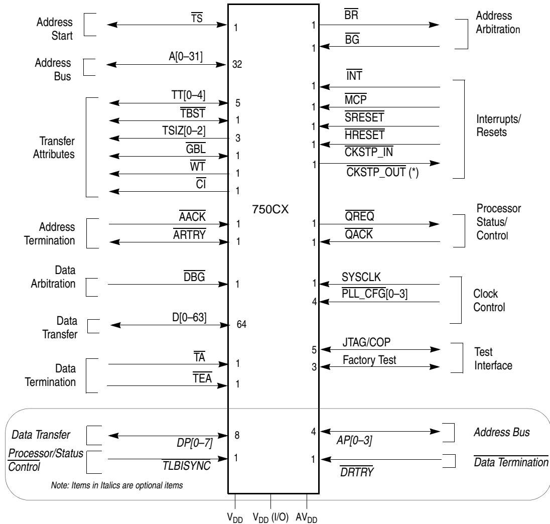
Figure 7-1. PowerPC 750CX Signal Groups
