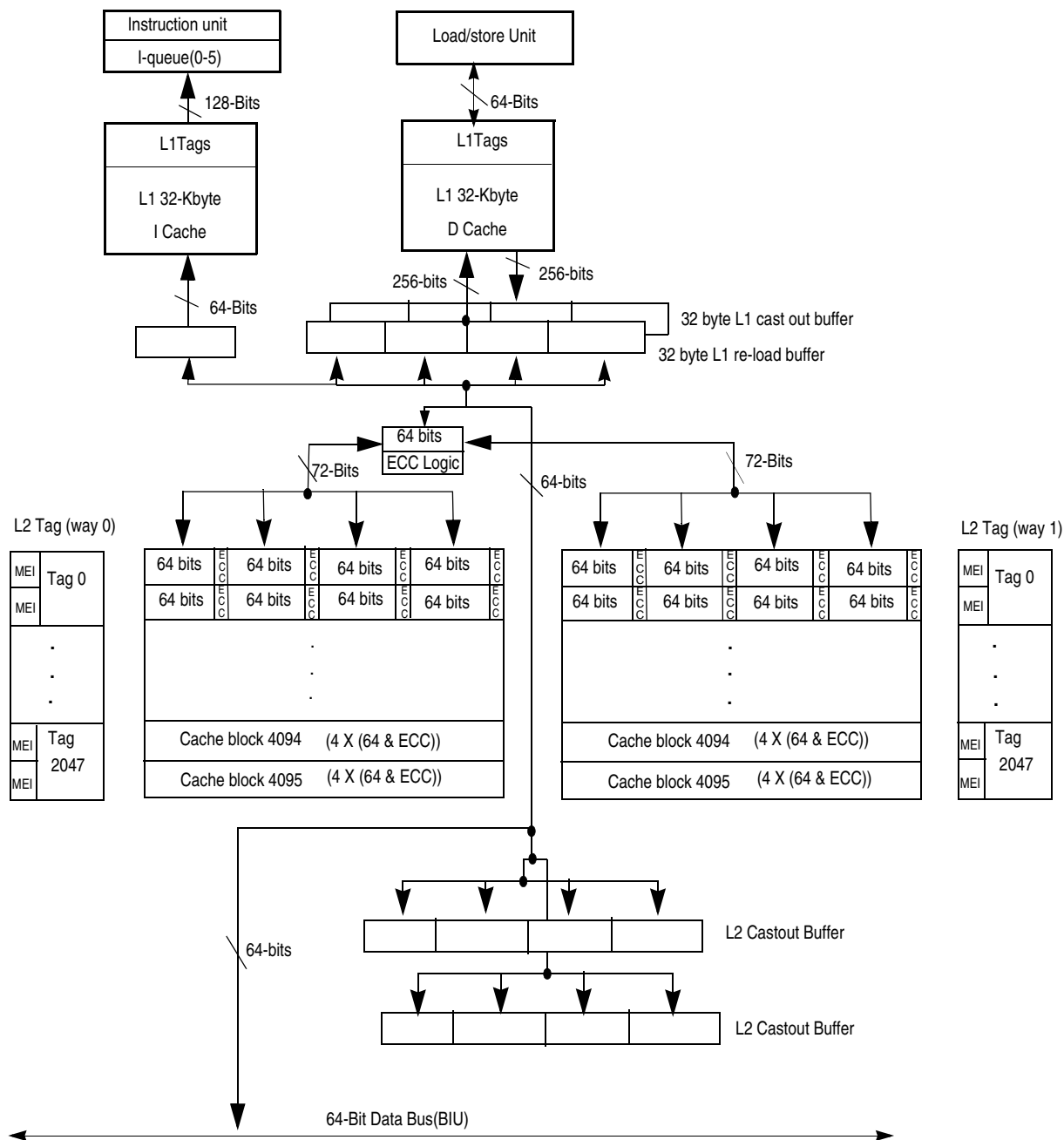
Figure 9-1. L2 Cache
