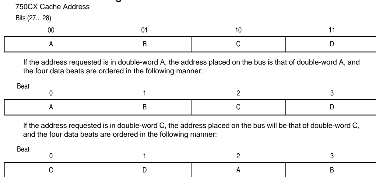
Figure 3-6. 750CX Cache Addresses
