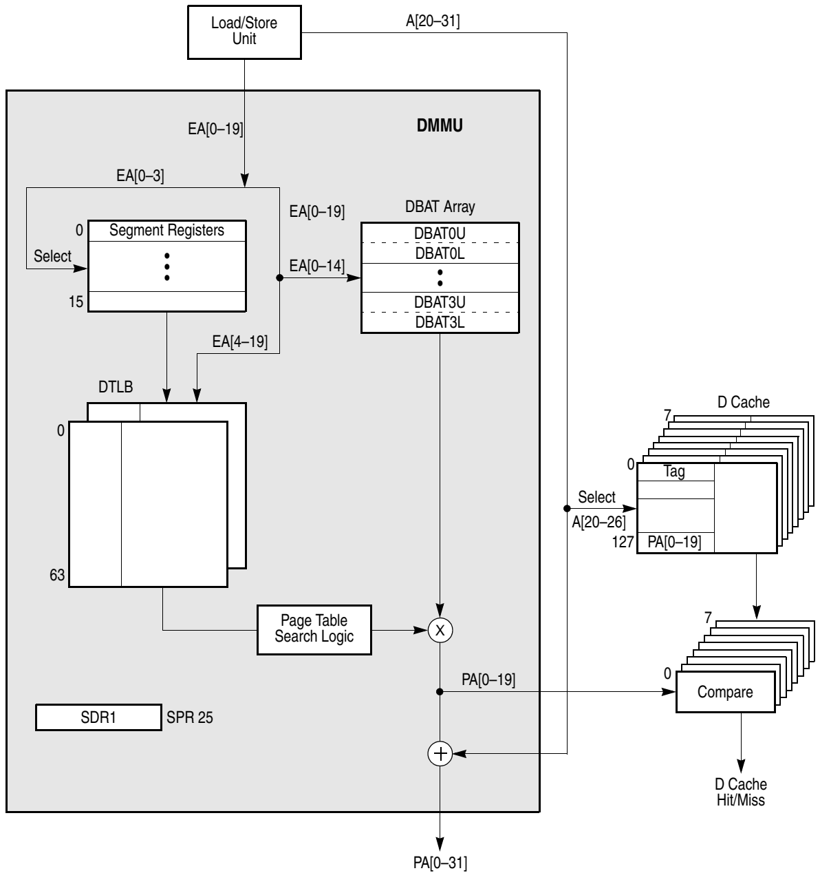
Figure 5-3. The 750CX Microprocessor DMMU Block Diagram
