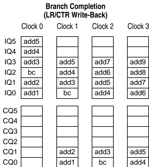
Figure 6-9. Branch Completion
