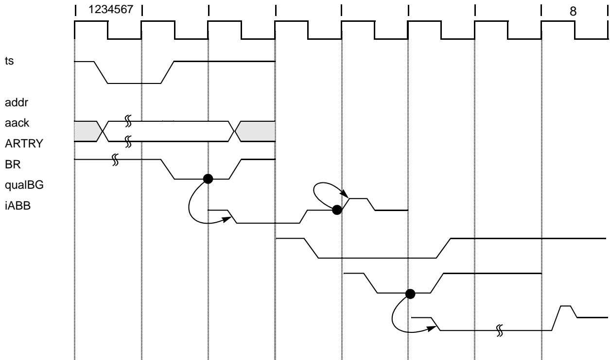
Figure 8-8. Snoop Address Cycle with \overline{ARTRY}
