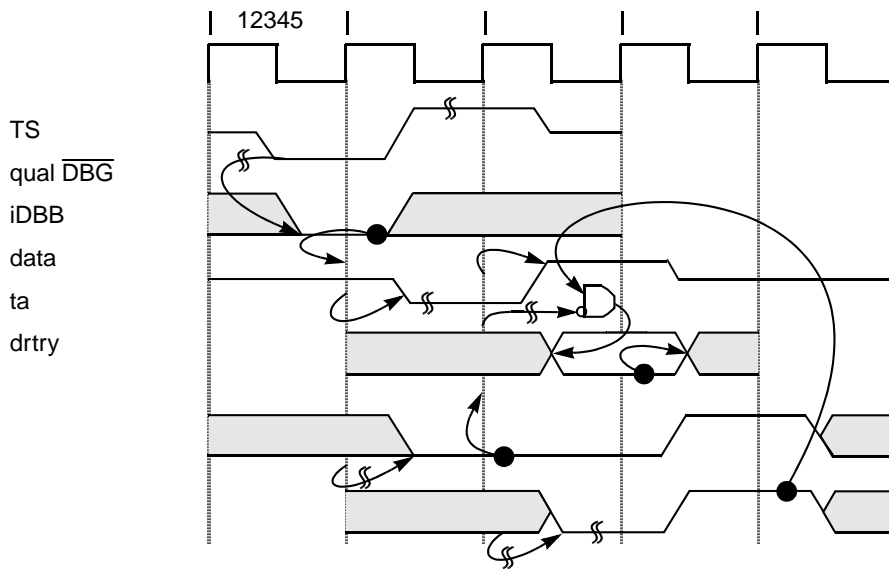
Figure 8-13. Termination with \overline{DRTRY}
