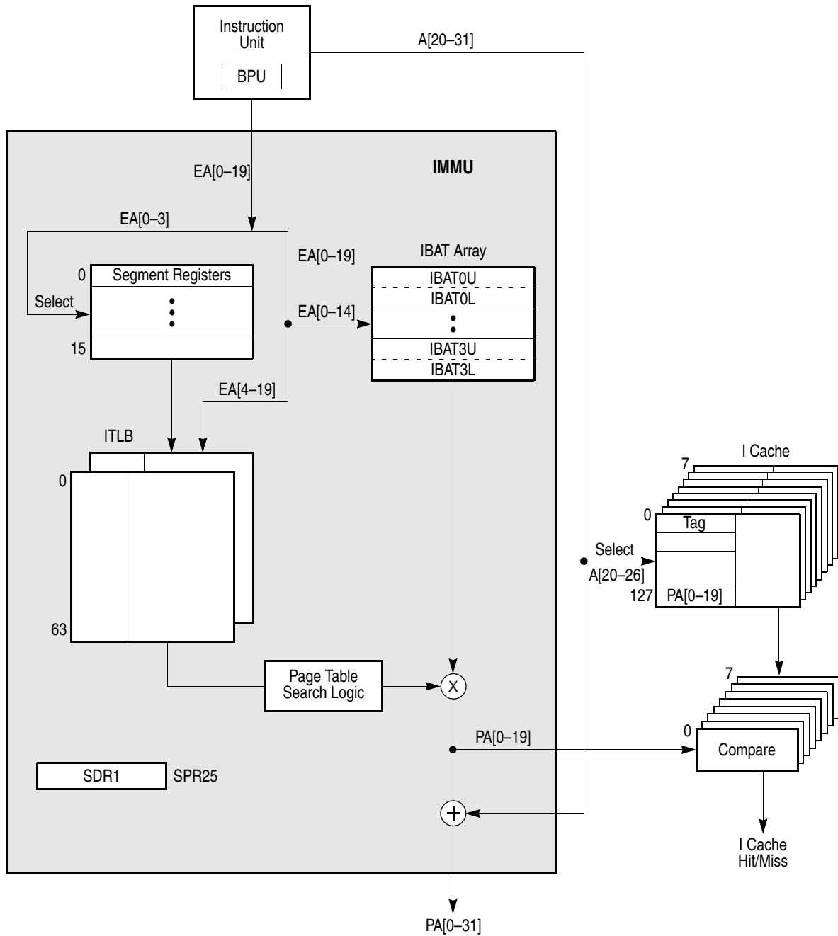
Figure 5-2. PowerPC 750CX Microprocessor IMMU Block Diagram
