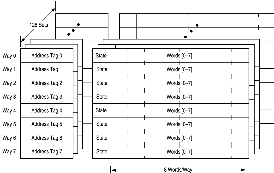
Figure 1-2. Cache Organization
