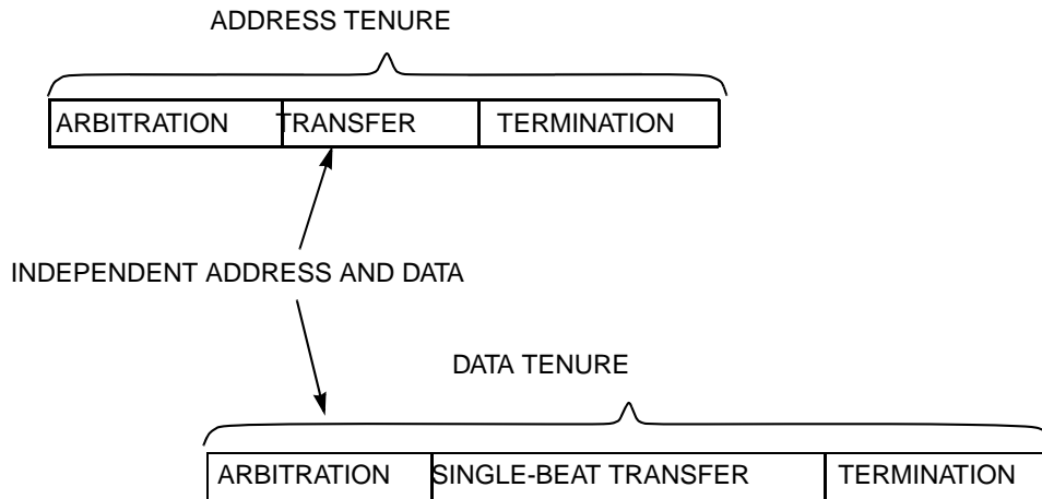
Figure 8-4. Overlapping Tenures on the 750CX Bus for a Single-Beat Transfer
